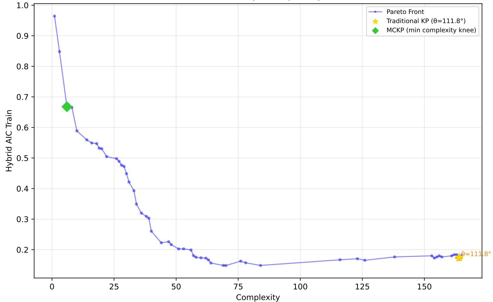
605_fri_c2_250_25 - Run 30 - MVP - Hybrid AIC Train \lambda_1=0.10, \lambda_2=0.00, \lambda_3=0.00 | Difficulty: 1.00 | Method: hmr
