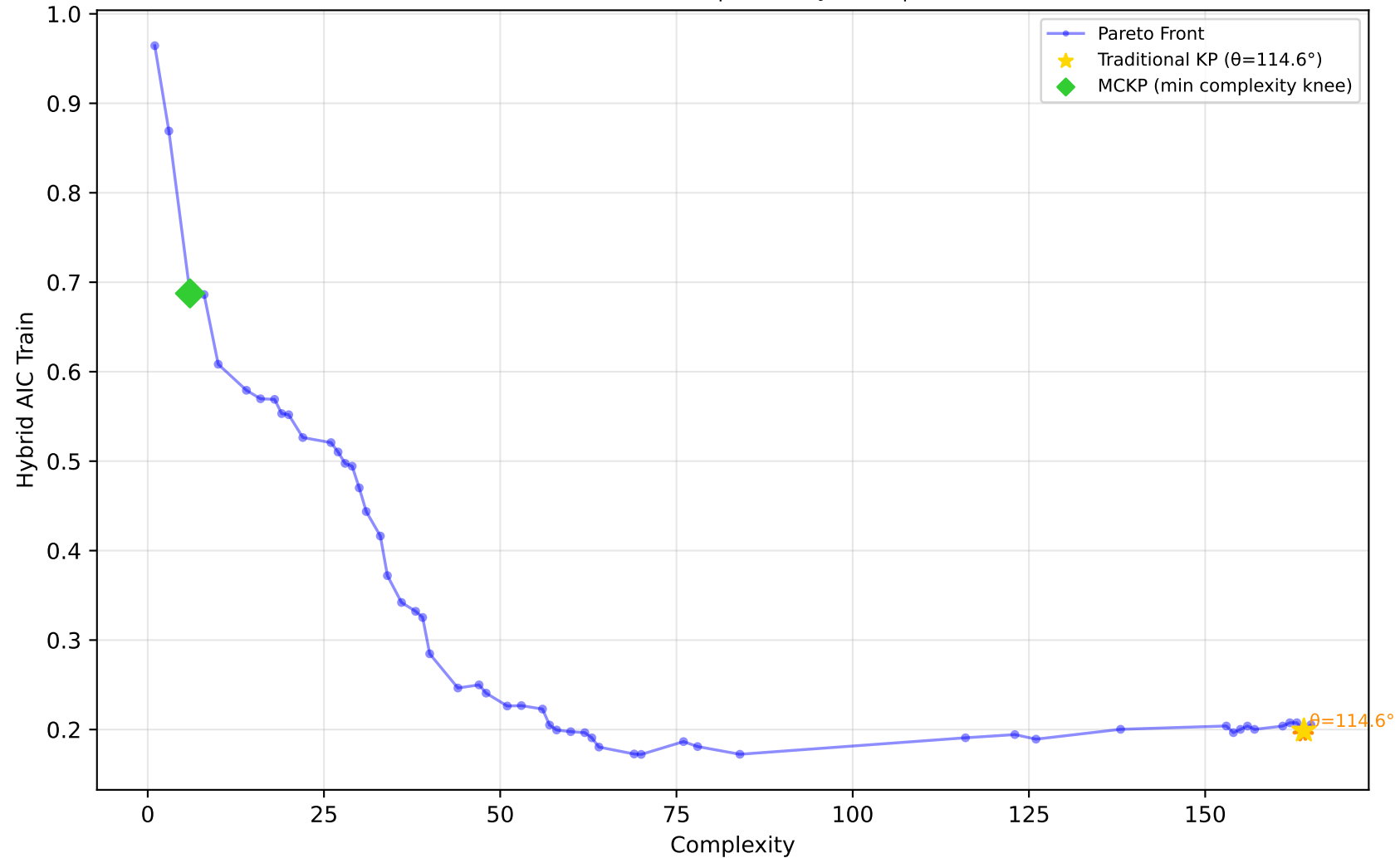
605_fri_c2_250_25 - Run 30 - MVP - Hybrid AIC Train \lambda_1=0.30, \lambda_2=0.00, \lambda_3=1.00 | Difficulty: 1.00 | Method: hmr
