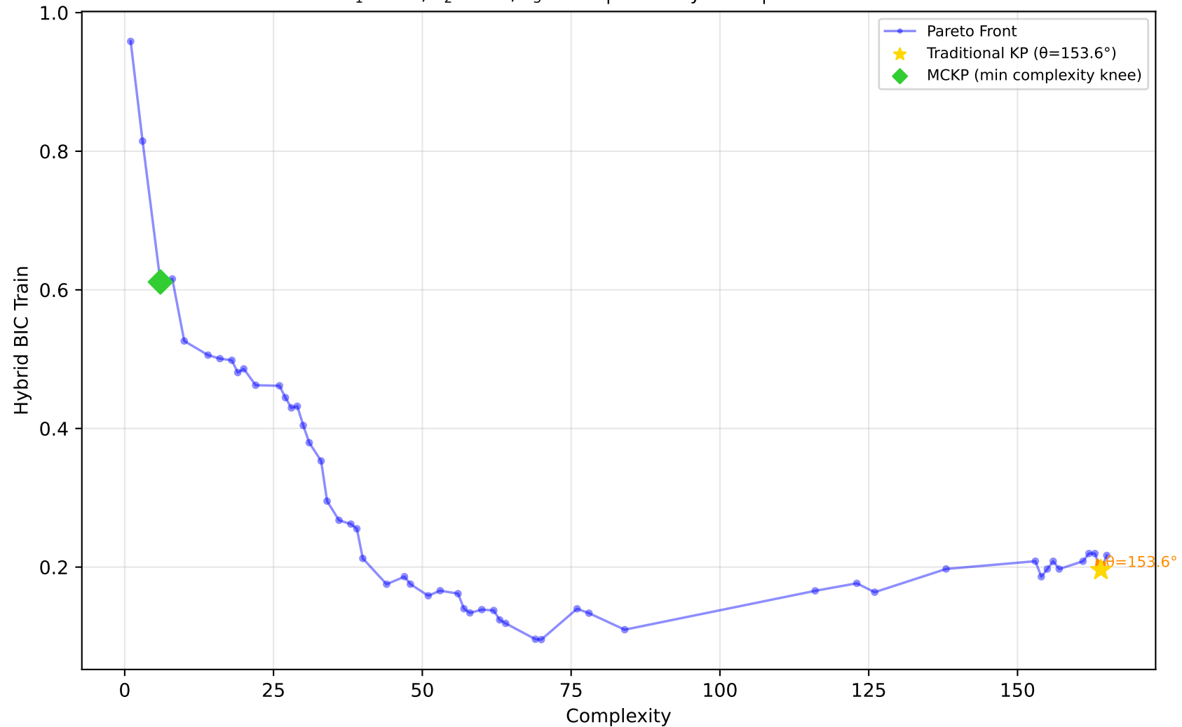
605_fri_c2_250_25 - Run 30 - MVP - Hybrid BIC Train \lambda_1=0.10, \lambda_2=0.00, \lambda_3=0.00 | Difficulty: 1.00 | Method: hmr
