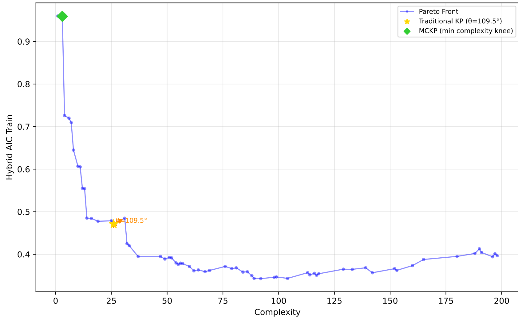
605_fri_c2_250_25 - Run 3 - MVP - Hybrid AIC Train \lambda_1=0.10, \lambda_2=0.00, \lambda_3=0.00 | Difficulty: 1.00 | Method: hmr
