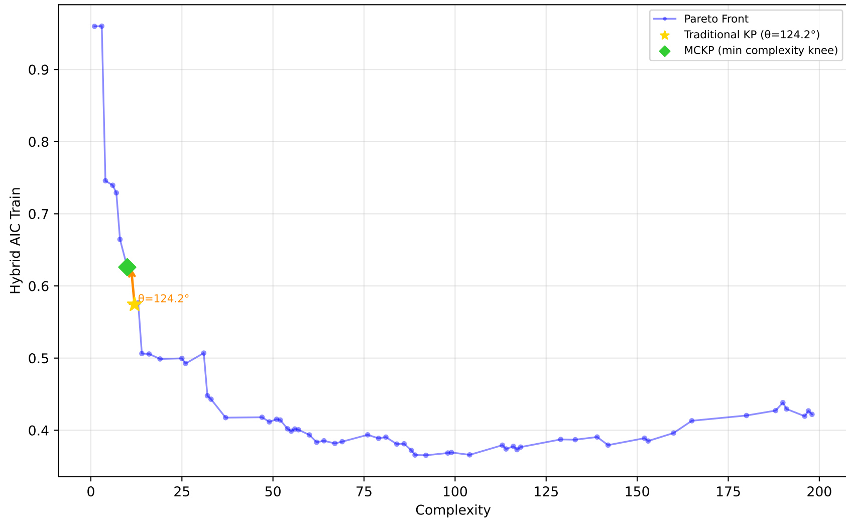
605_fri_c2_250_25 - Run 3 - MVP - Hybrid AIC Train \lambda_1=0.30 , \lambda_2=0.00 , \lambda_3=1.00 | Difficulty: 1.00 | Method: hmr
