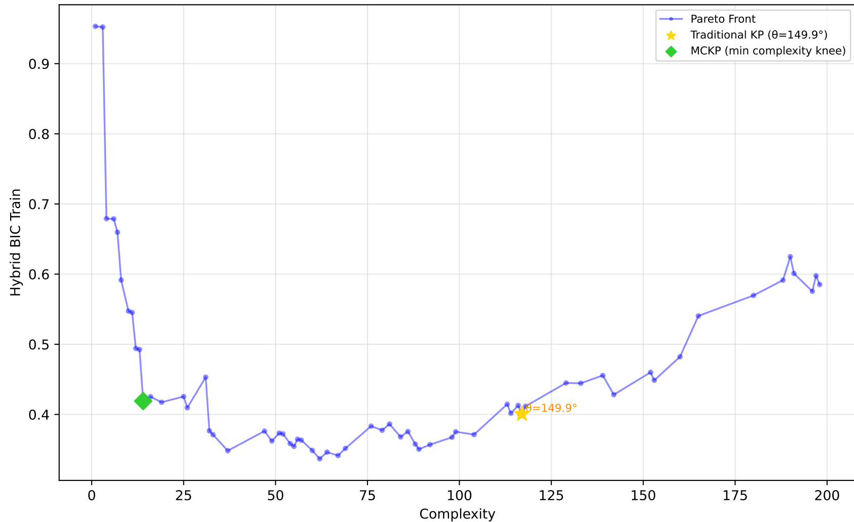
605_fri_c2_250_25 - Run 3 - MVP - Hybrid BIC Train \lambda_1=0.10, \lambda_2=0.00, \lambda_3=0.00 | Difficulty: 1.00 | Method: hmr
