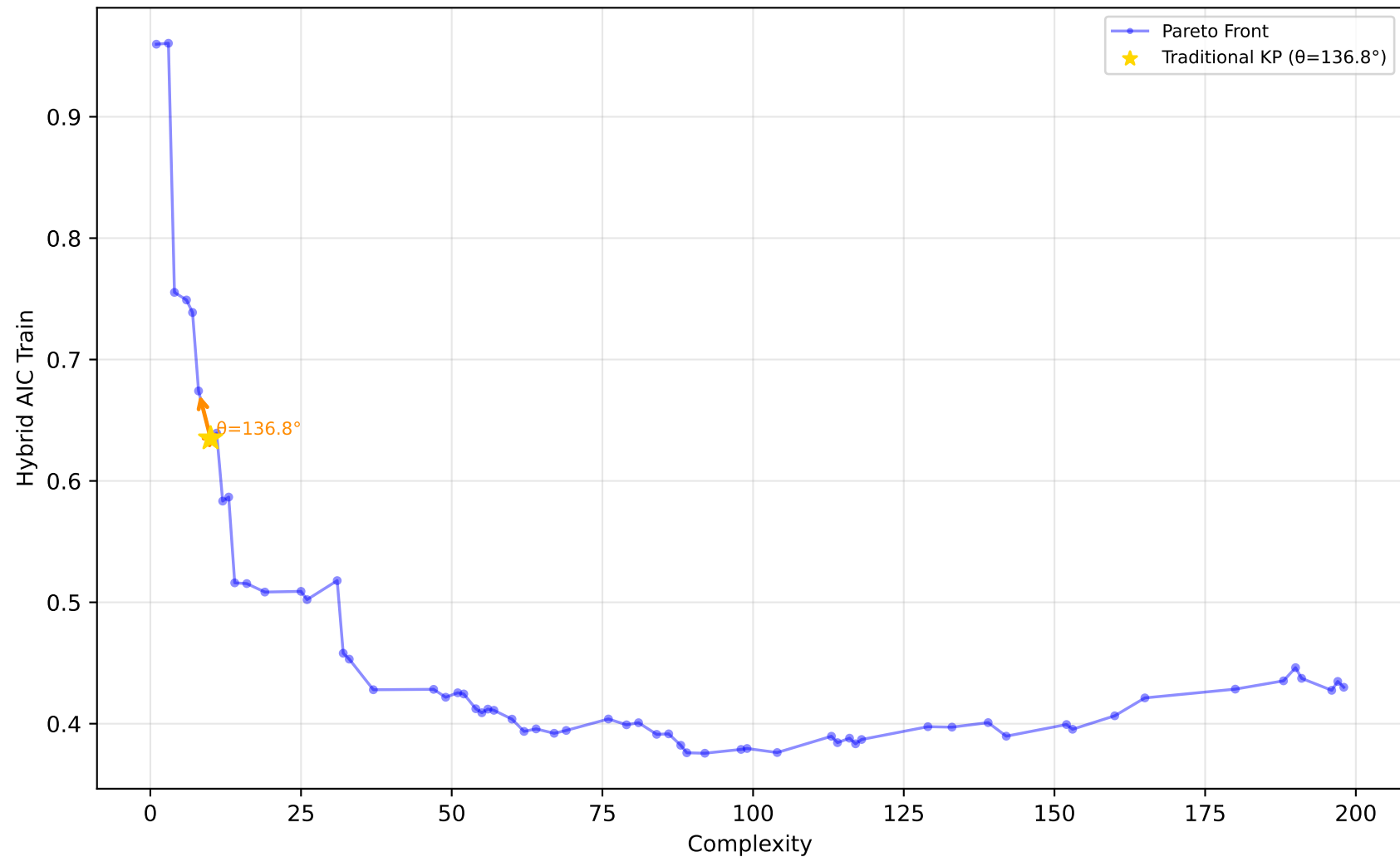
605_fri_c2_250_25 - Run 3 - SVP - Hybrid AIC Train \lambda_1=0.40, \lambda_2=0.00, \lambda_3=0.20 | Difficulty: 1.00 | Method: hmr
