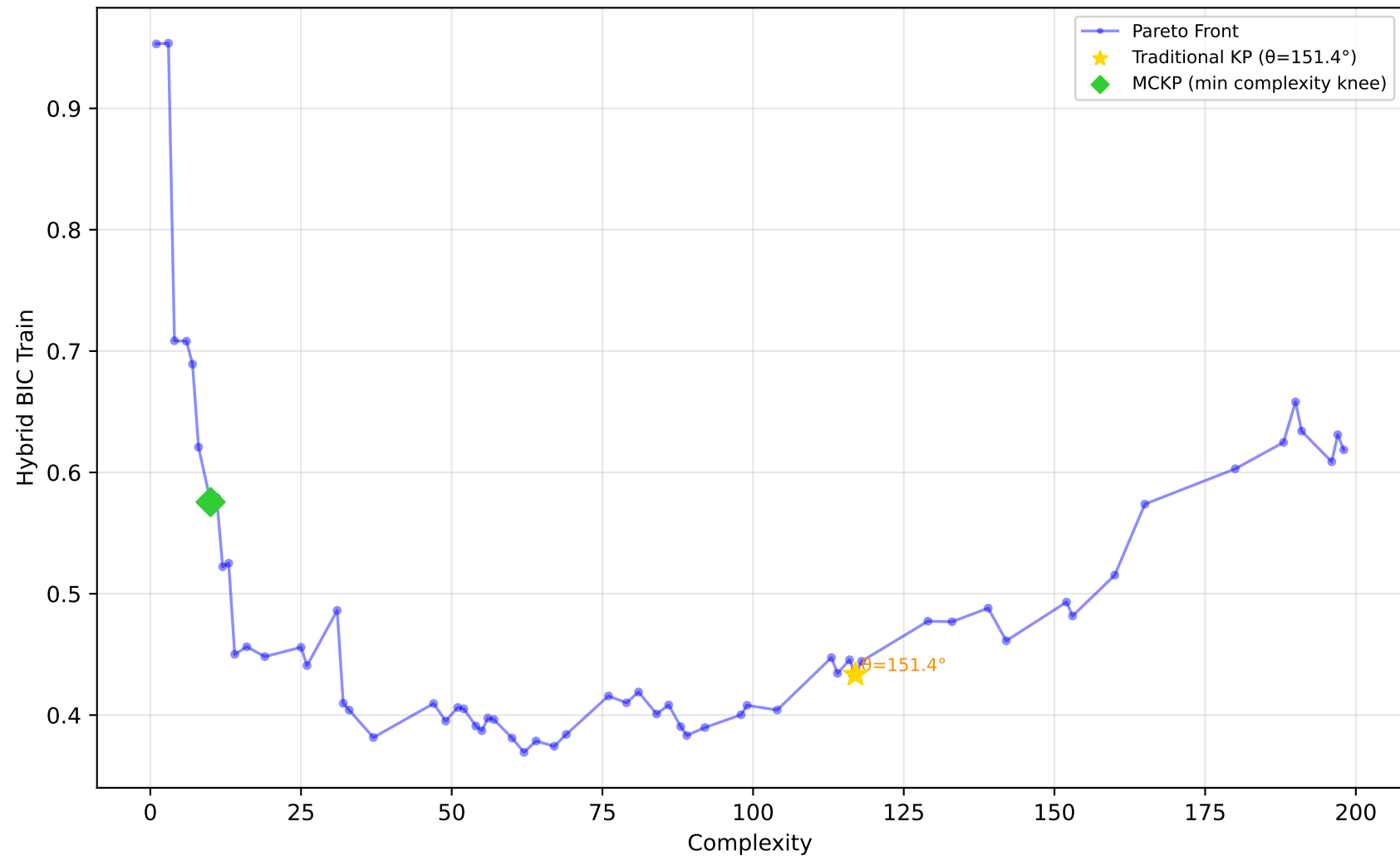
605_fri_c2_250_25 - Run 3 - SVP - Hybrid BIC Train \lambda_1=0.40, \lambda_2=0.00, \lambda_3=0.20 | Difficulty: 1.00 | Method: hmr
