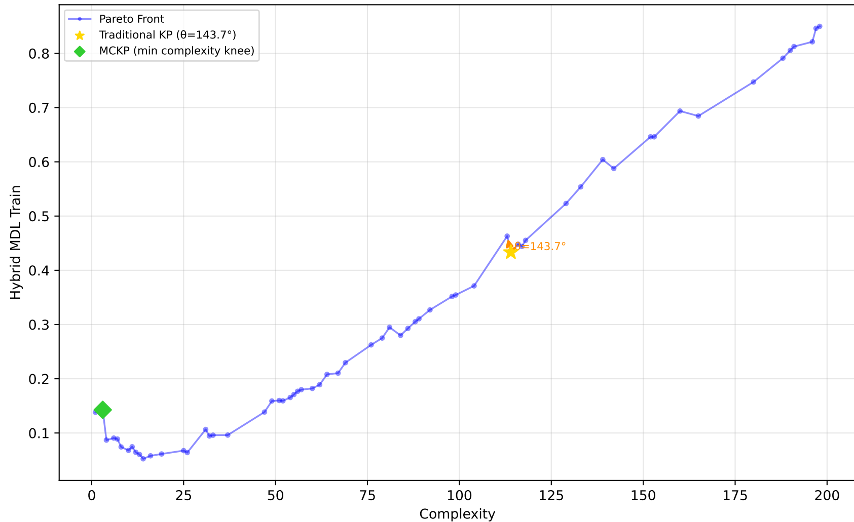
605_fri_c2_250_25 - Run 3 - SVP - Hybrid MDL Train \lambda_1=0.10, \lambda_2=0.00, \lambda_3=0.00 | Difficulty: 1.00 | Method: hmr
