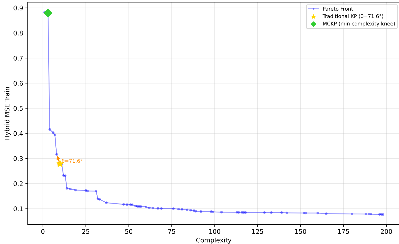
605_fri_c2_250_25 - Run 3 - SVP - Hybrid MSE Train \lambda_1=0.10, \lambda_2=0.00, \lambda_3=0.00 | Difficulty: 1.00 | Method: hmr
