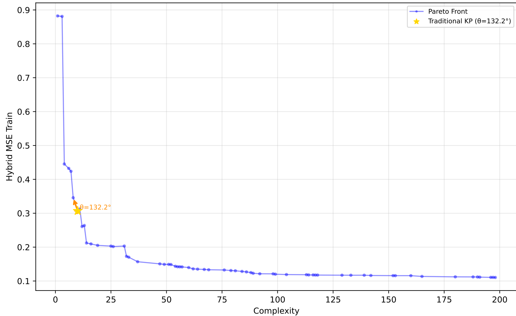
605_fri_c2_250_25 - Run 3 - SVP - Hybrid MSE Train \lambda_1=0.40, \lambda_2=0.00, \lambda_3=0.20 | Difficulty: 1.00 | Method: hmr
