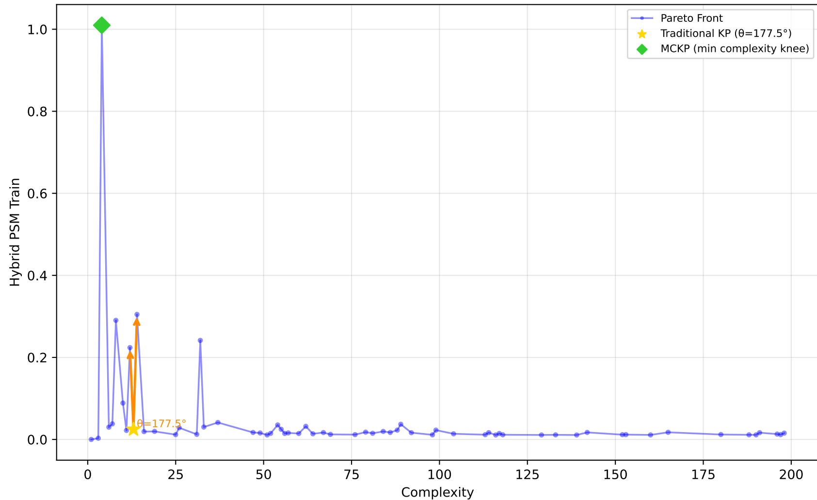
605_fri_c2_250_25 - Run 3 - SVP - Hybrid PSM Train \lambda_1=0.10, \lambda_2=0.00, \lambda_3=0.00 | Difficulty: 1.00 | Method: hmr
