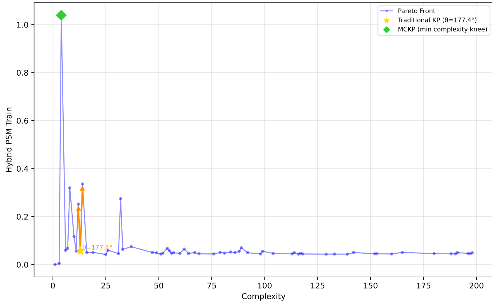
605_fri_c2_250_25 - Run 3 - SVP - Hybrid PSM Train \lambda_1=0.40, \lambda_2=0.00, \lambda_3=0.20 | Difficulty: 1.00 | Method: hmr
