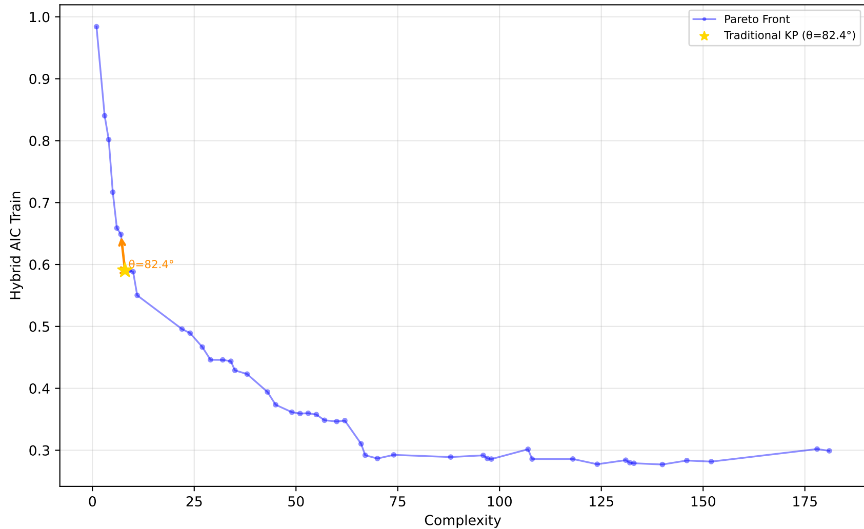
605_fri_c2_250_25 - Run 4 - MVP - Hybrid AIC Train \lambda_1=0.10, \lambda_2=0.00, \lambda_3=0.00 | Difficulty: 1.00 | Method: hmr
