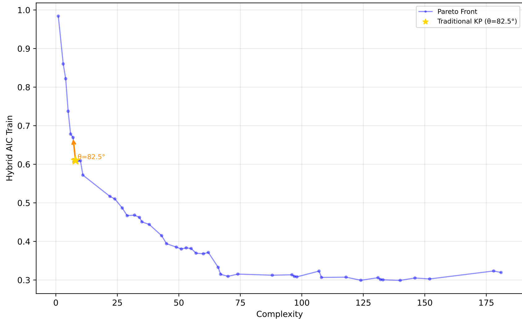
605_fri_c2_250_25 - Run 4 - MVP - Hybrid AIC Train \lambda_1=0.30, \lambda_2=0.00, \lambda_3=1.00 | Difficulty: 1.00 | Method: hmr
