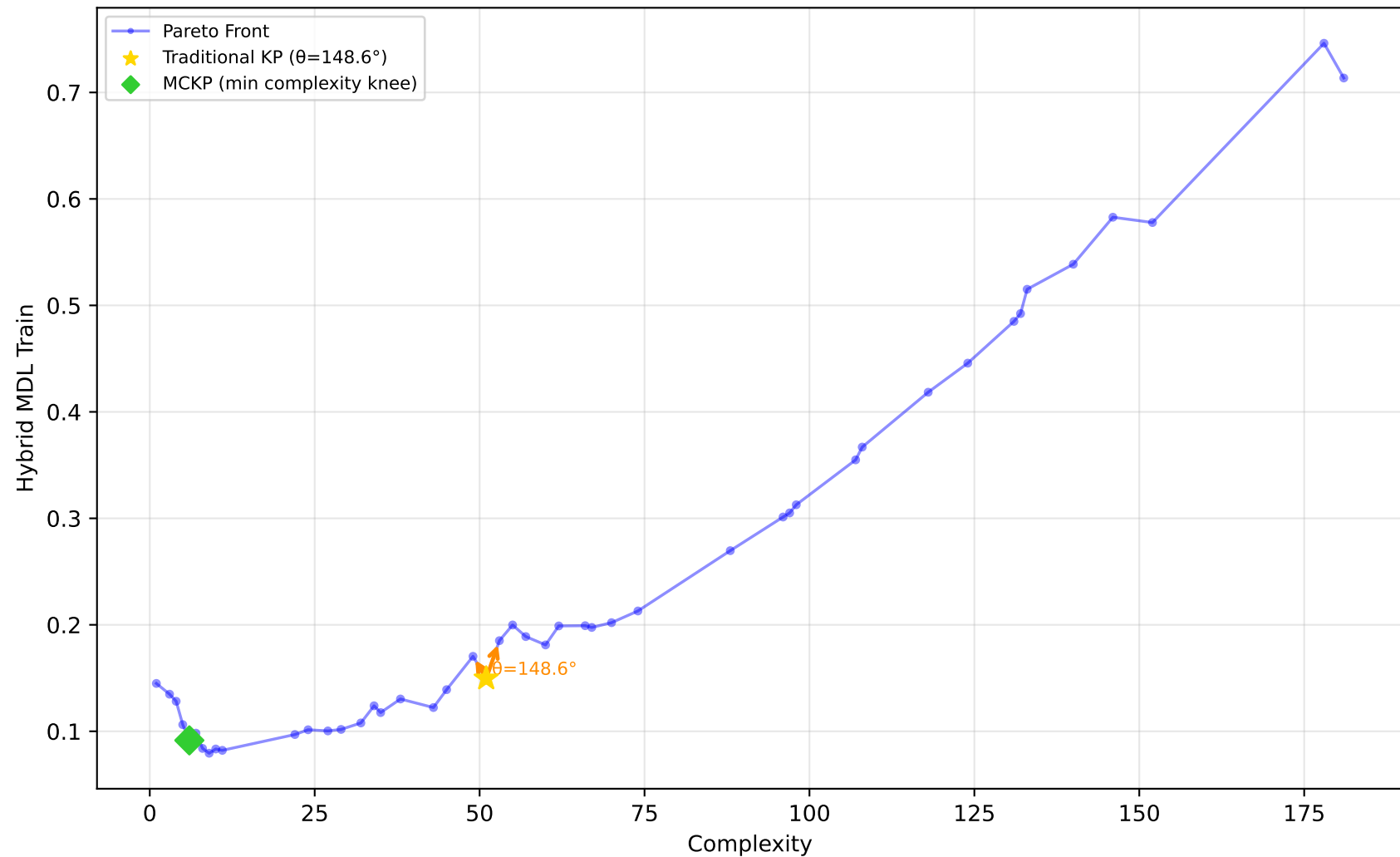
605_fri_c2_250_25 - Run 4 - MVP - Hybrid MDL Train \lambda_1=0.30, \lambda_2=0.00, \lambda_3=1.00 | Difficulty: 1.00 | Method: hmr
