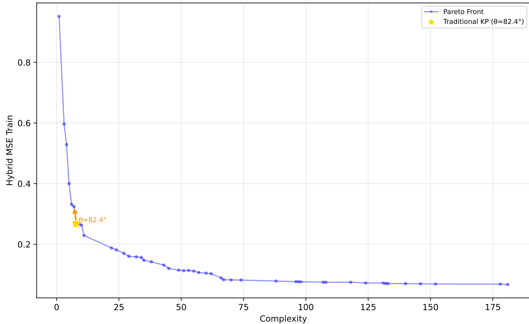
605_fri_c2_250_25 - Run 4 - MVP - Hybrid MSE Train \lambda_1=0.10, \lambda_2=0.00, \lambda_3=0.00 | Difficulty: 1.00 | Method: hmr
