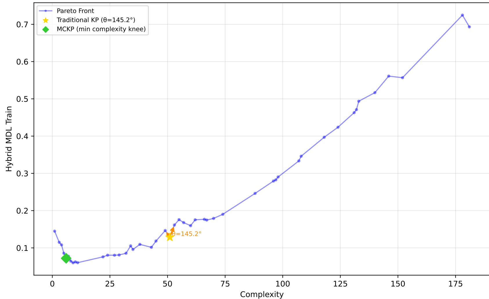
605_fri_c2_250_25 - Run 4 - SVP - Hybrid MDL Train \lambda_1=0.10, \lambda_2=0.00, \lambda_3=0.00 | Difficulty: 1.00 | Method: hmr
