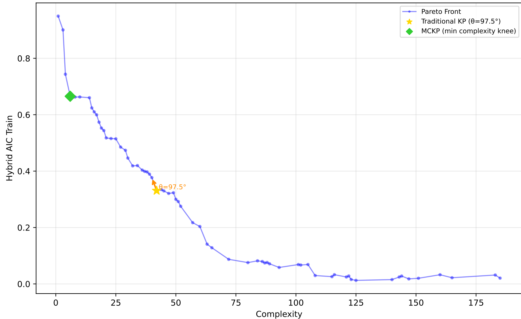
605_fri_c2_250_25 - Run 5 - MVP - Hybrid AIC Train \lambda_1=0.10, \lambda_2=0.00, \lambda_3=0.00 | Difficulty: 1.00 | Method: hmr
