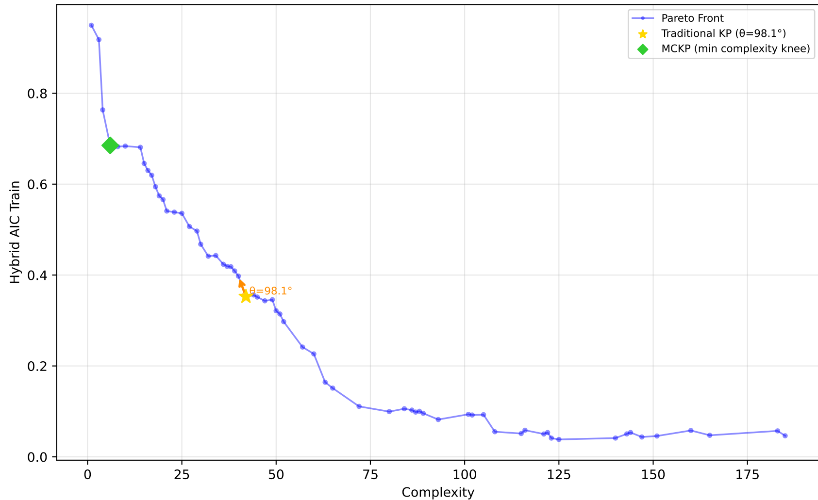
605_fri_c2_250_25 - Run 5 - MVP - Hybrid AIC Train \lambda_1=0.30, \lambda_2=0.00, \lambda_3=1.00 | Difficulty: 1.00 | Method: hmr
