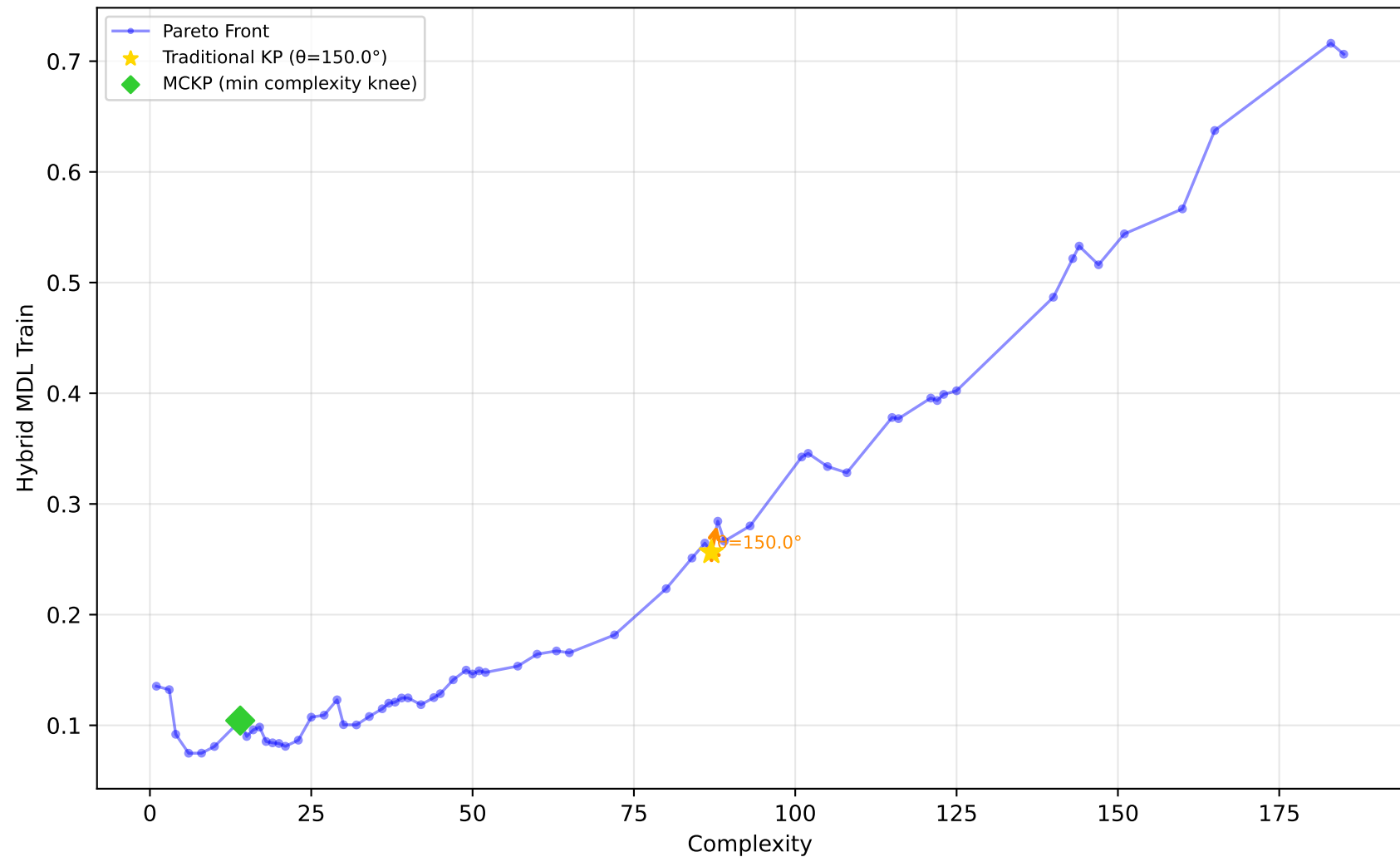
605_fri_c2_250_25 - Run 5 - MVP - Hybrid MDL Train \lambda_1=0.10, \lambda_2=0.00, \lambda_3=0.00 | Difficulty: 1.00 | Method: hmr
