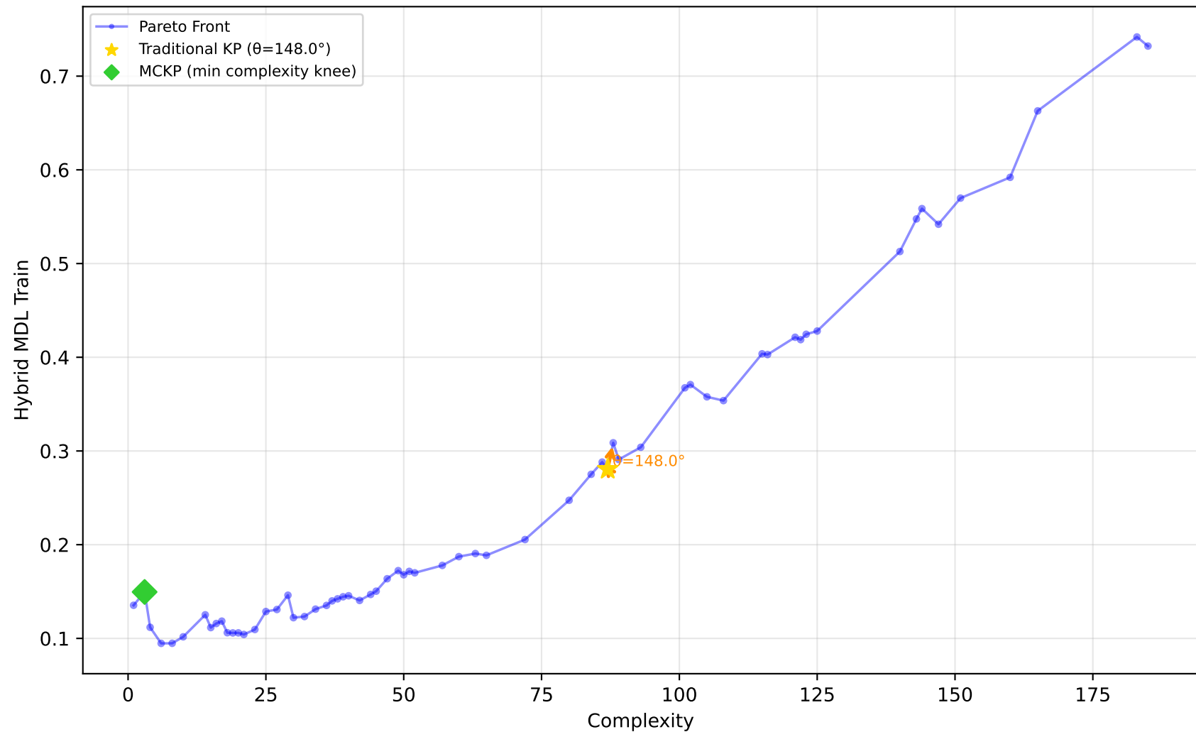
605_fri_c2_250_25 - Run 5 - MVP - Hybrid MDL Train \lambda_1=0.30, \lambda_2=0.00, \lambda_3=1.00 | Difficulty: 1.00 | Method: hmr
