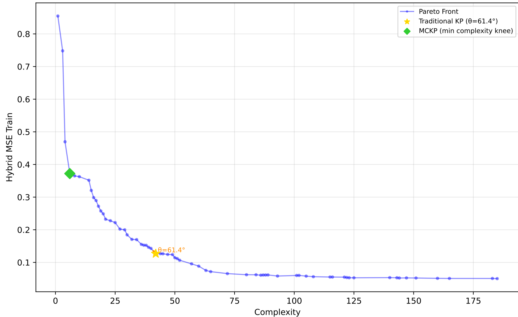
605_fri_c2_250_25 - Run 5 - SVP - Hybrid MSE Train \lambda_1=0.40 , \lambda_2=0.00 , \lambda_3=0.20 | Difficulty: 1.00 | Method: hmr
