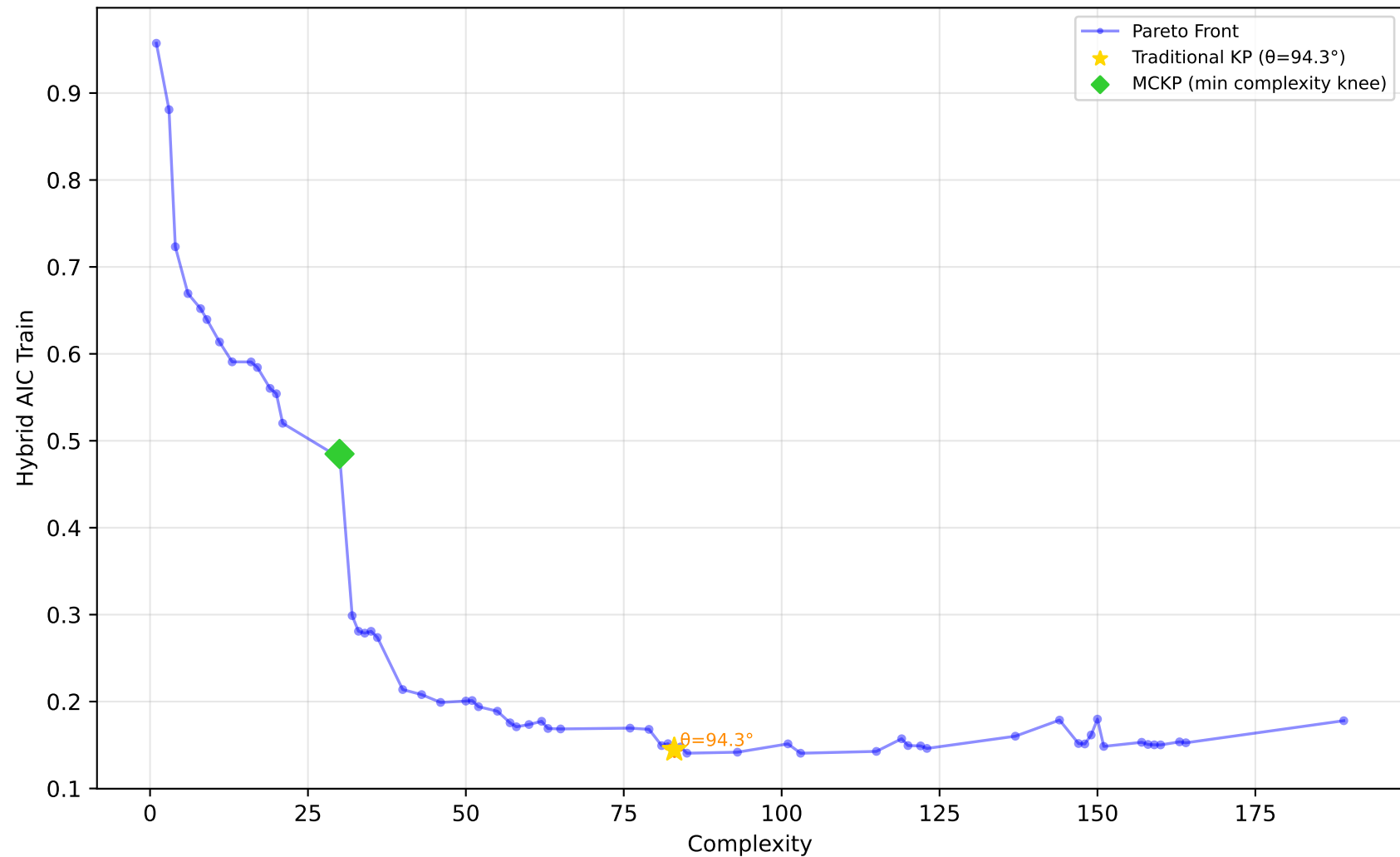
605_fri_c2_250_25 - Run 6 - MVP - Hybrid AIC Train \lambda_1=0.30, \lambda_2=0.00, \lambda_3=1.00 | Difficulty: 1.00 | Method: hmr
