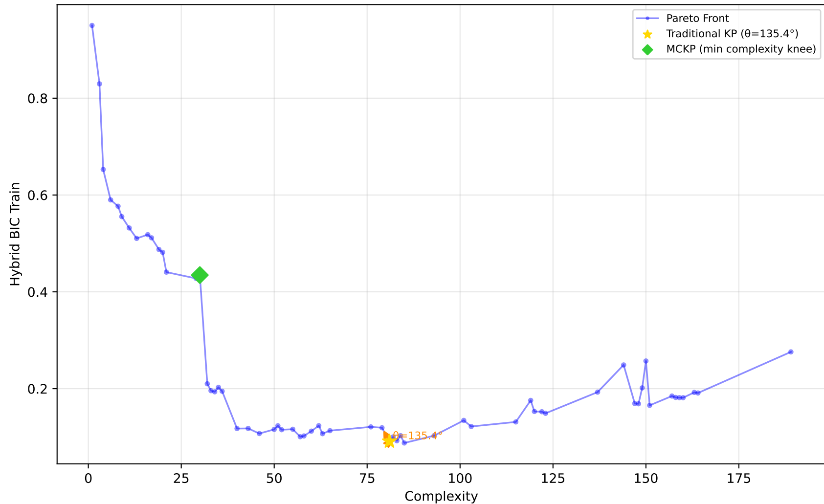
605_fri_c2_250_25 - Run 6 - MVP - Hybrid BIC Train \lambda_1=0.10, \lambda_2=0.00, \lambda_3=0.00 | Difficulty: 1.00 | Method: hmr
