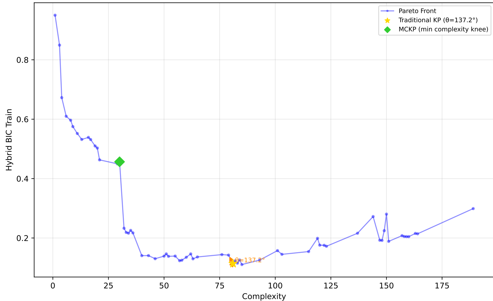
605_fri_c2_250_25 - Run 6 - MVP - Hybrid BIC Train \lambda_1=0.30, \lambda_2=0.00, \lambda_3=1.00 | Difficulty: 1.00 | Method: hmr
