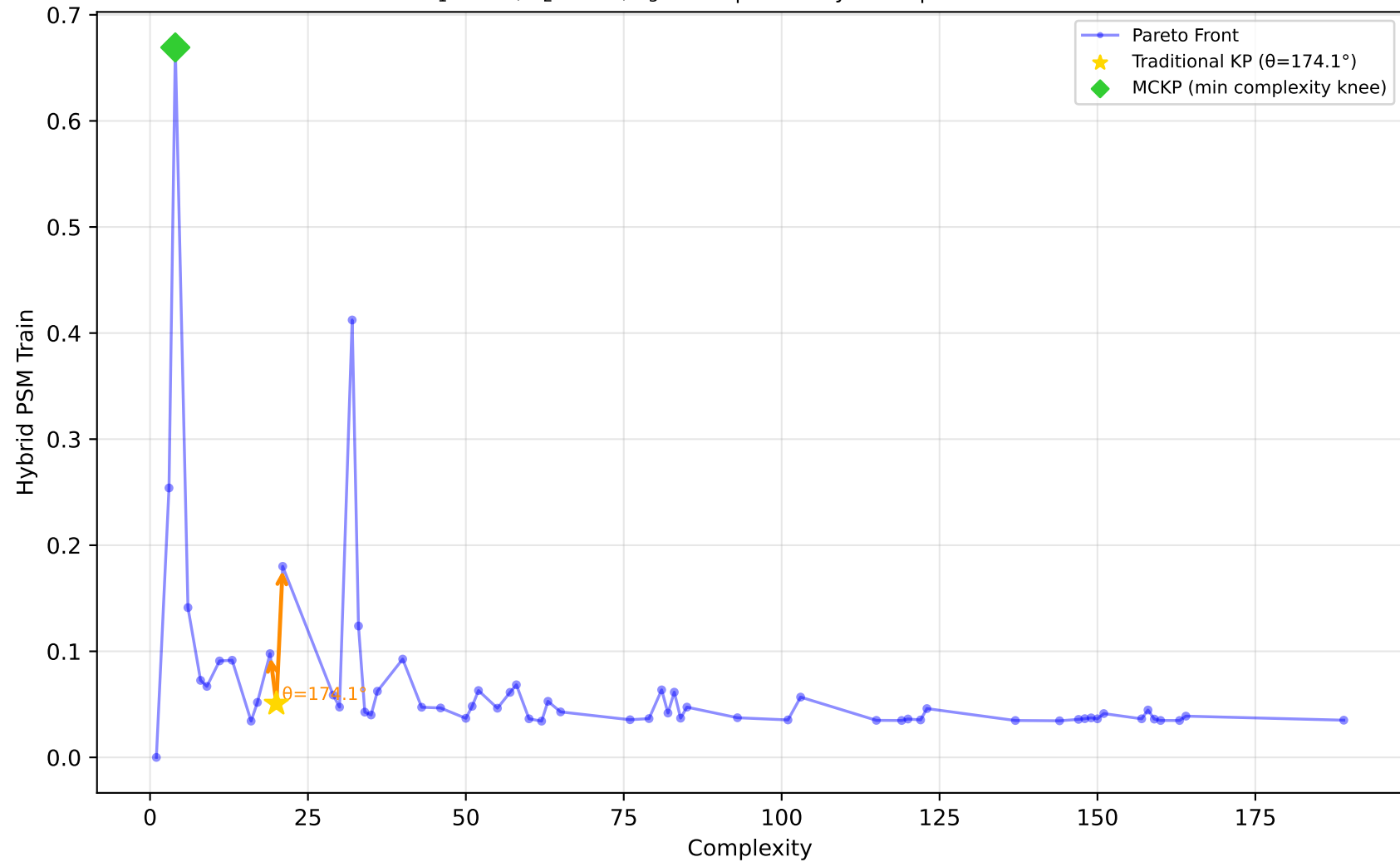
605_fri_c2_250_25 - Run 6 - MVP - Hybrid PSM Train \lambda_1=0.30, \lambda_2=0.00, \lambda_3=1.00 | Difficulty: 1.00 | Method: hmr
