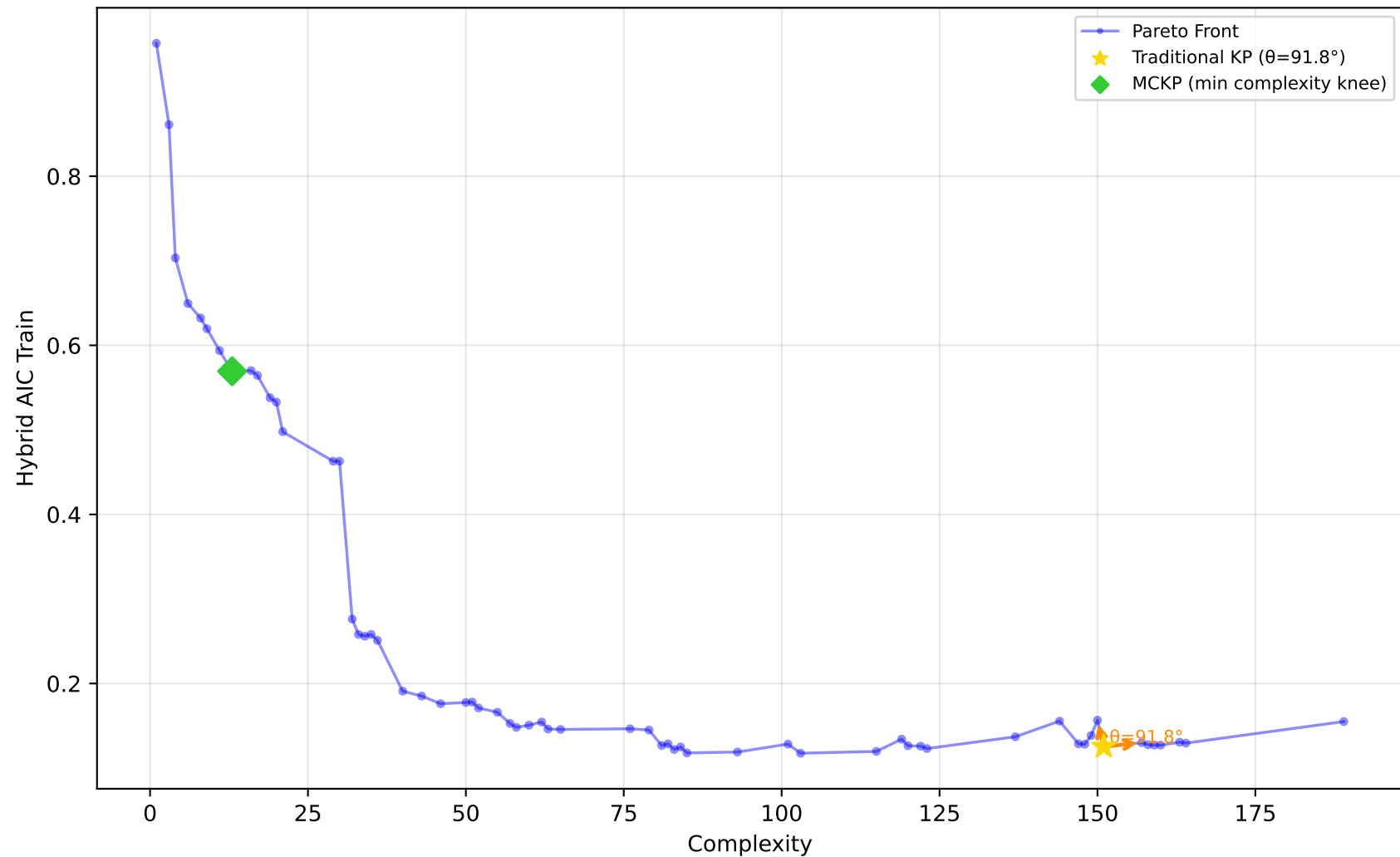
605_fri_c2_250_25 - Run 6 - SVP - Hybrid AIC Train \lambda_1=0.10, \lambda_2=0.00, \lambda_3=0.00 | Difficulty: 1.00 | Method: hmr
