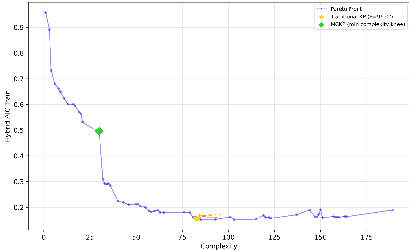
605_fri_c2_250_25 - Run 6 - SVP - Hybrid AIC Train \lambda_1=0.40, \lambda_2=0.00, \lambda_3=0.20 | Difficulty: 1.00 | Method: hmr
