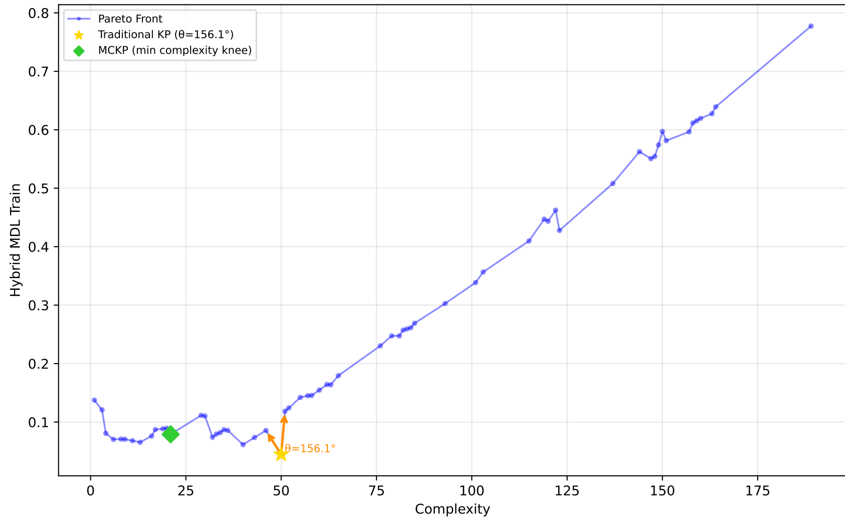
605_fri_c2_250_25 - Run 6 - SVP - Hybrid MDL Train \lambda_1=0.10, \lambda_2=0.00, \lambda_3=0.00 | Difficulty: 1.00 | Method: hmr
