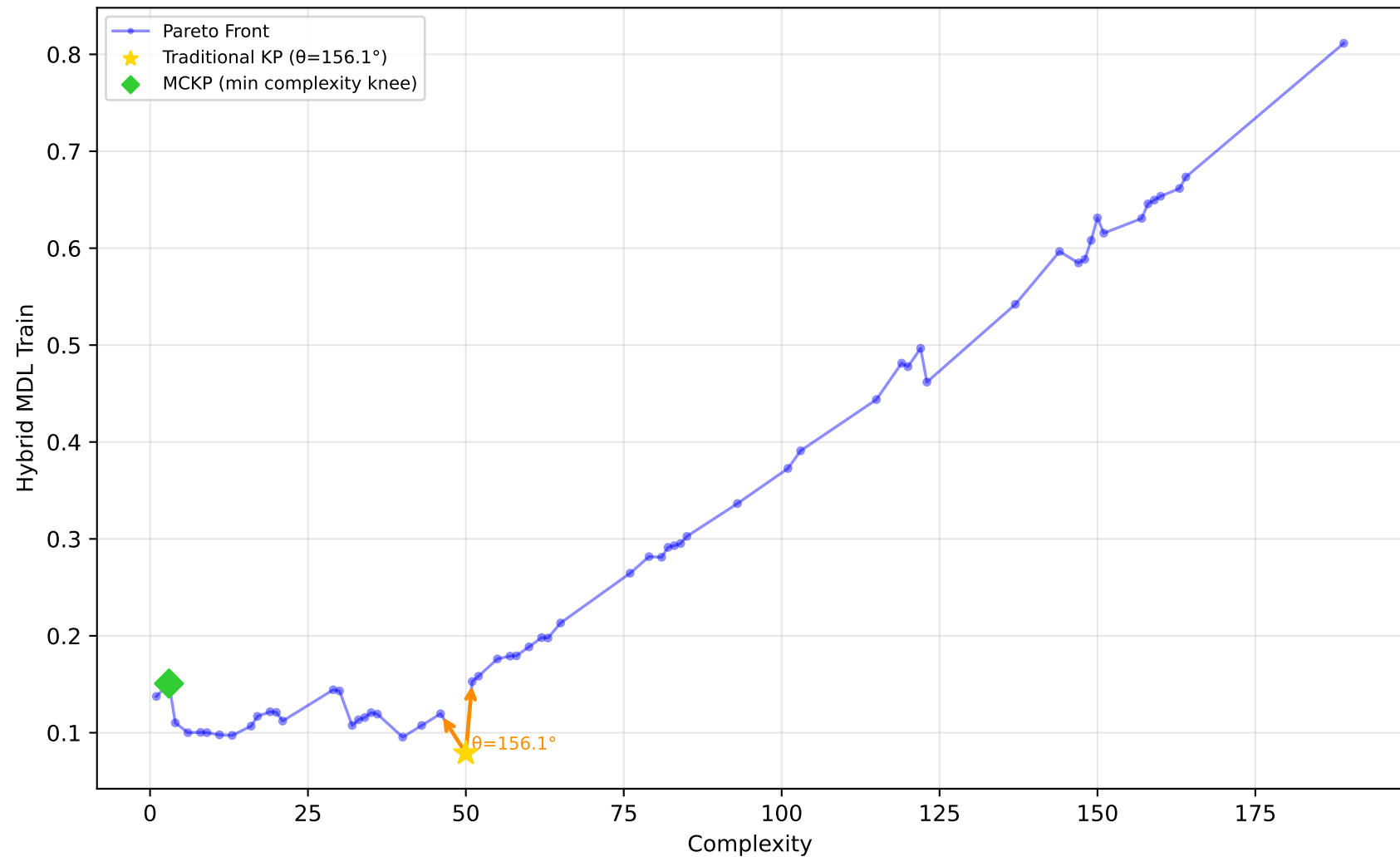
605_fri_c2_250_25 - Run 6 - SVP - Hybrid MDL Train \lambda_1=0.40, \lambda_2=0.00, \lambda_3=0.20 | Difficulty: 1.00 | Method: hmr
