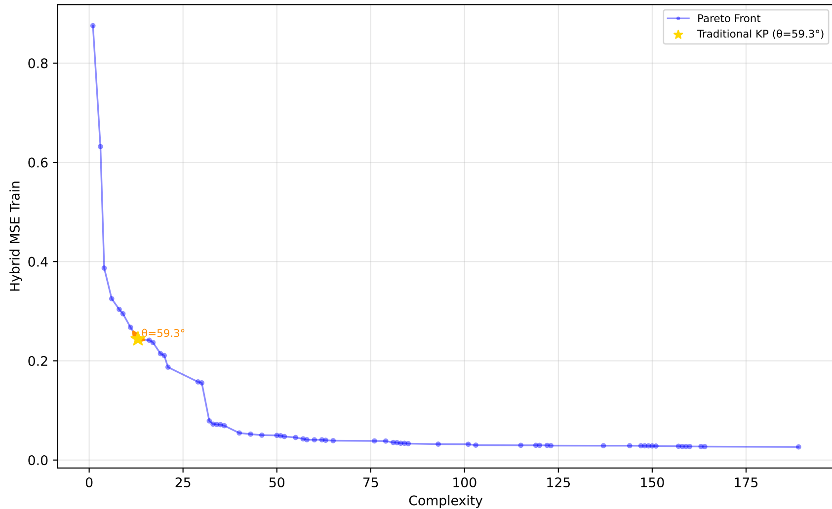
605_fri_c2_250_25 - Run 6 - SVP - Hybrid MSE Train \lambda_1=0.10, \lambda_2=0.00, \lambda_3=0.00 | Difficulty: 1.00 | Method: hmr
