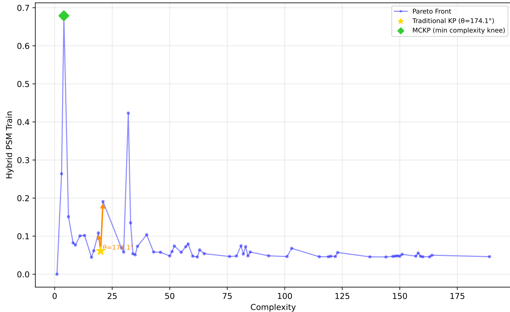
605_fri_c2_250_25 - Run 6 - SVP - Hybrid PSM Train \lambda_1=0.40, \lambda_2=0.00, \lambda_3=0.20 | Difficulty: 1.00 | Method: hmr
