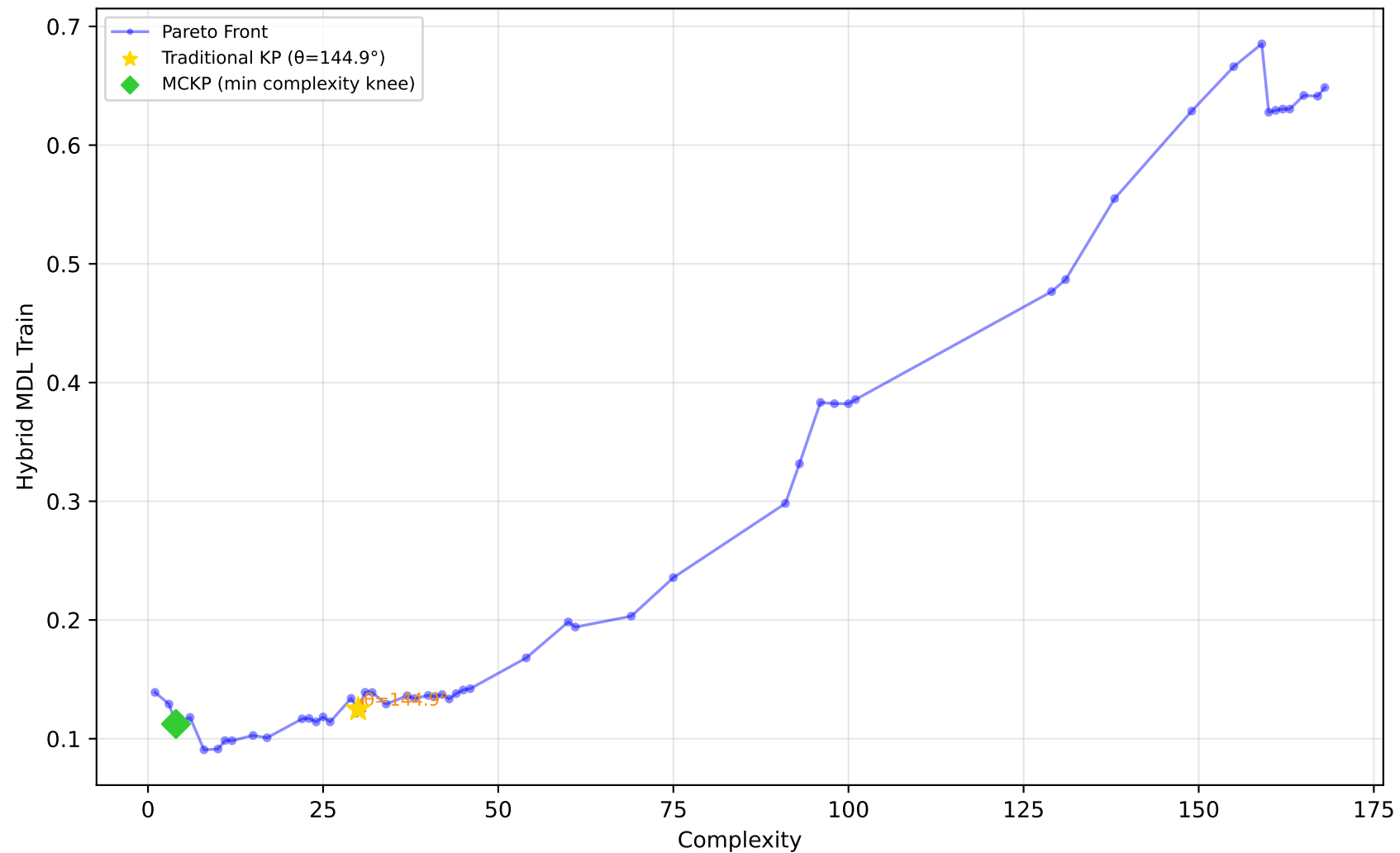
605_fri_c2_250_25 - Run 7 - MVP - Hybrid MDL Train \lambda_1=0.30 , \lambda_2=0.00 , \lambda_3=1.00 | Difficulty: 1.00 | Method: hmr
