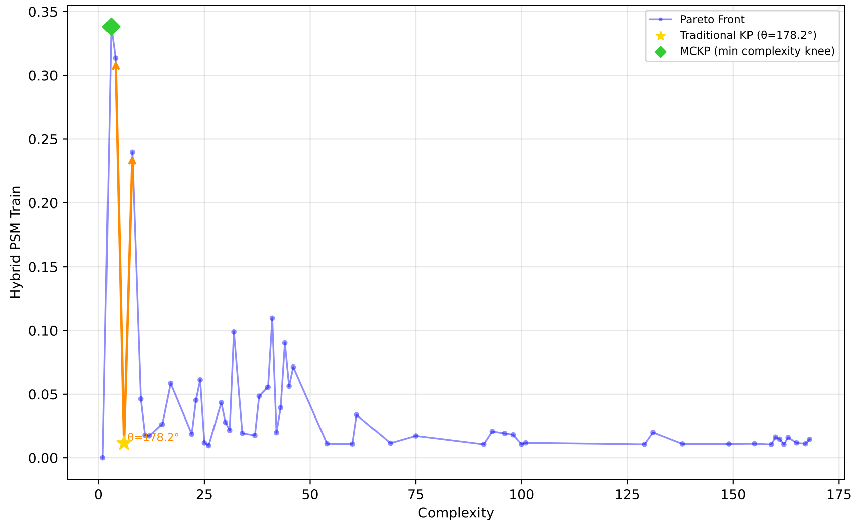
605_fri_c2_250_25 - Run 7 - MVP - Hybrid PSM Train \lambda_1=0.10, \lambda_2=0.00, \lambda_3=0.00 | Difficulty: 1.00 | Method: hmr
