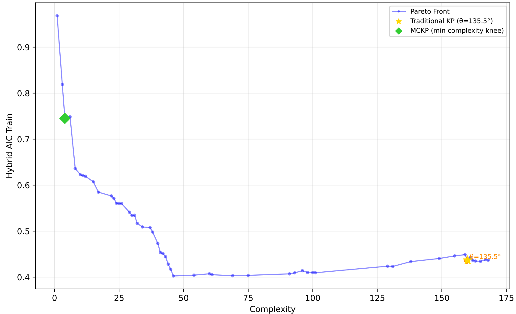
605_fri_c2_250_25 - Run 7 - SVP - Hybrid AIC Train \lambda_1=0.10, \lambda_2=0.00, \bar{\lambda}_3=0.00 | Difficulty: 1.00 | Method: hmr
