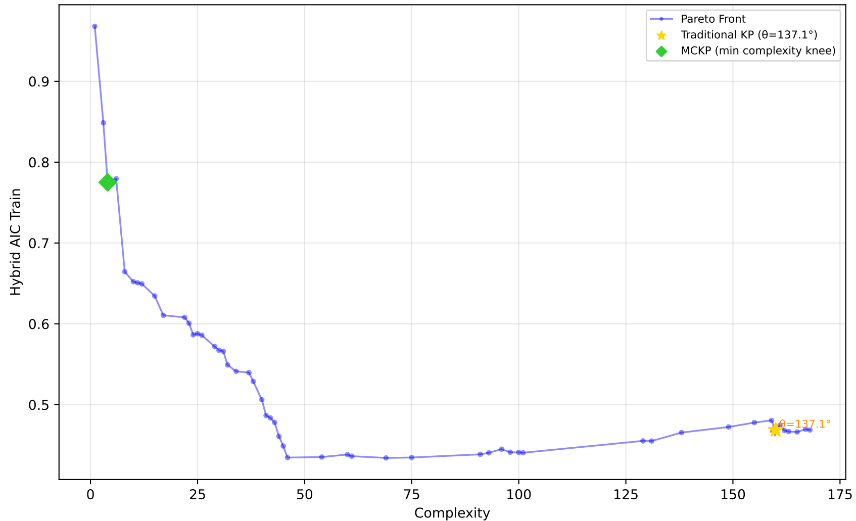
605_fri_c2_250_25 - Run 7 - SVP - Hybrid AIC Train \lambda_1=0.40 , \lambda_2=0.00 , \lambda_3=0.20 | Difficulty: 1.00 | Method: hmr
