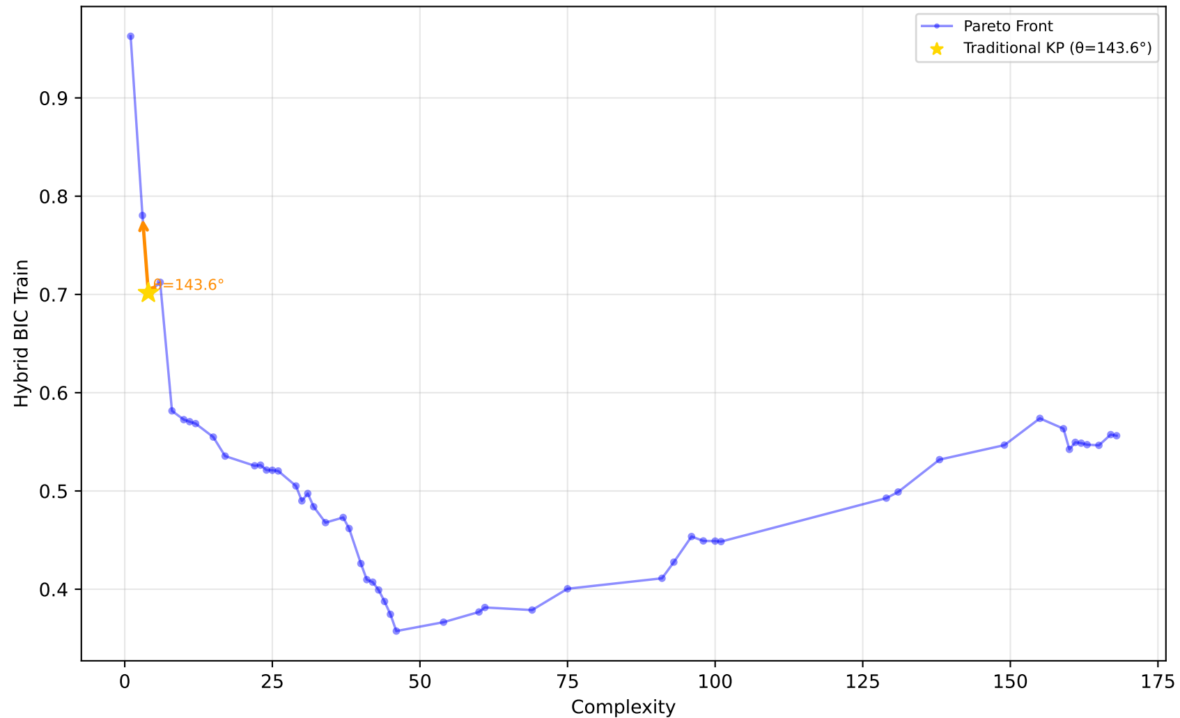
605_fri_c2_250_25 - Run 7 - SVP - Hybrid BIC Train \lambda_1=0.10, \lambda_2=0.00, \lambda_3=0.00 | Difficulty: 1.00 | Method: hmr
