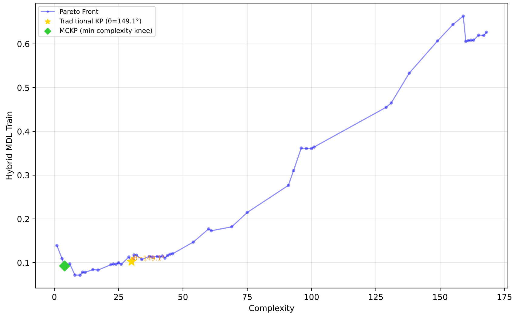
605_fri_c2_250_25 - Run 7 - SVP - Hybrid MDL Train \lambda_1=0.10, \lambda_2=0.00, \lambda_3=0.00 | Difficulty: 1.00 | Method: hmr
