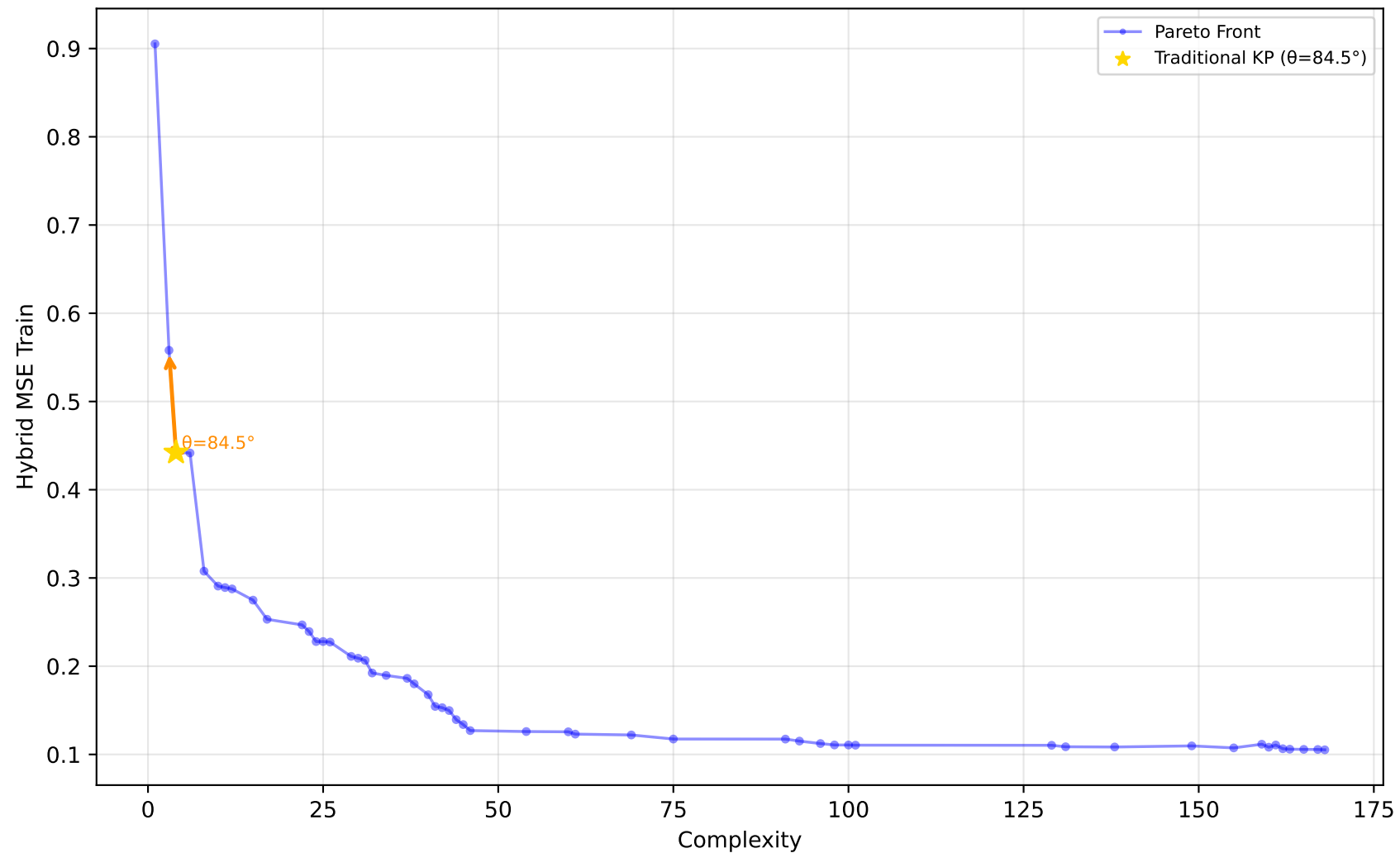
605_fri_c2_250_25 - Run 7 - SVP - Hybrid MSE Train \lambda_1=0.10, \lambda_2=0.00, \lambda_3=0.00 | Difficulty: 1.00 | Method: hmr
