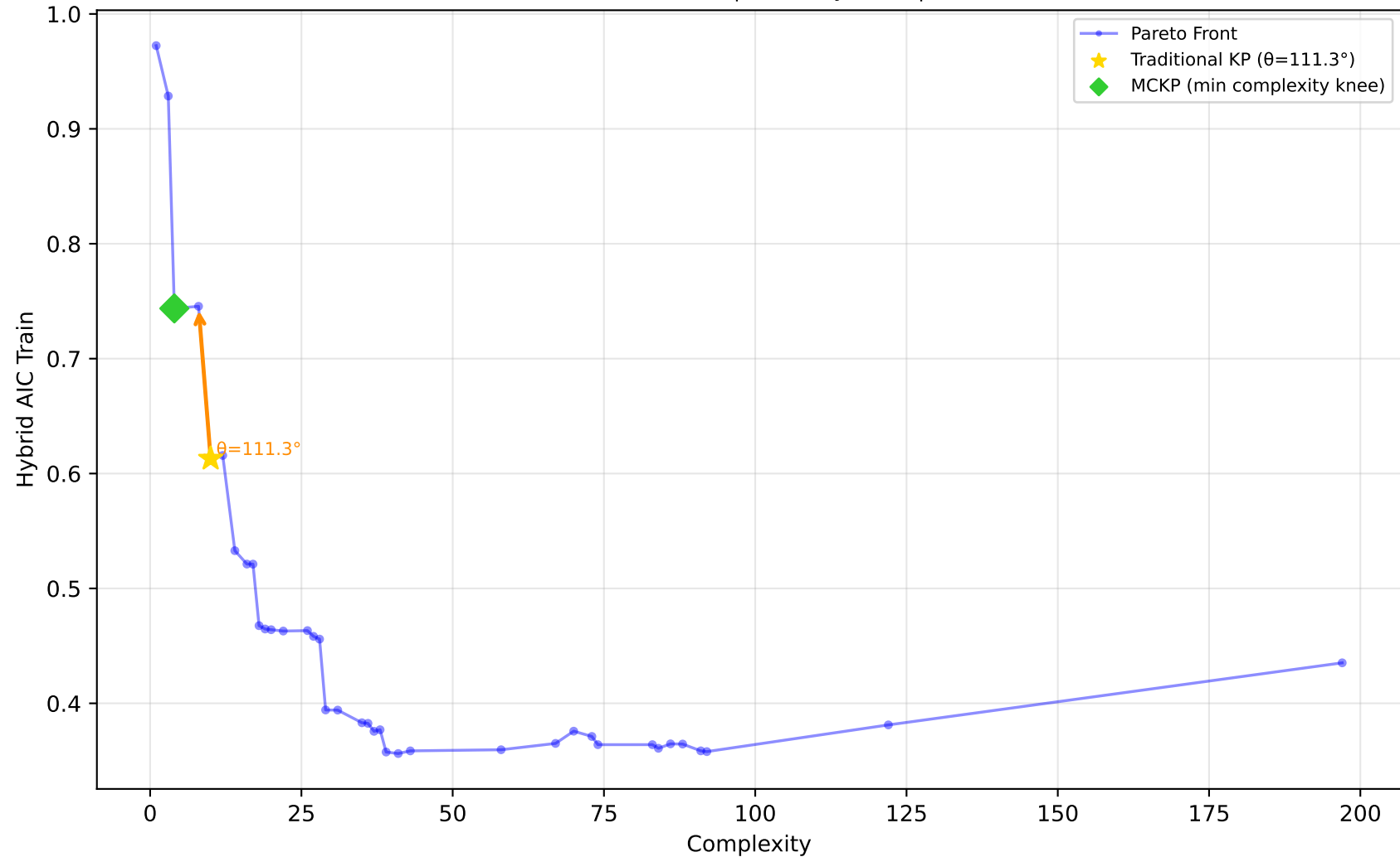
605_fri_c2_250_25 - Run 8 - MVP - Hybrid AIC Train \lambda_1=0.10, \lambda_2=0.00, \lambda_3=0.00 | Difficulty: 1.00 | Method: hmr
