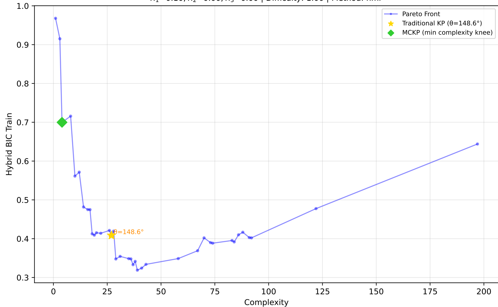
605_fri_c2_250_25 - Run 8 - MVP - Hybrid BIC Train \lambda_1=0.10, \lambda_2=0.00, \lambda_3=0.00 | Difficulty: 1.00 | Method: hmr
