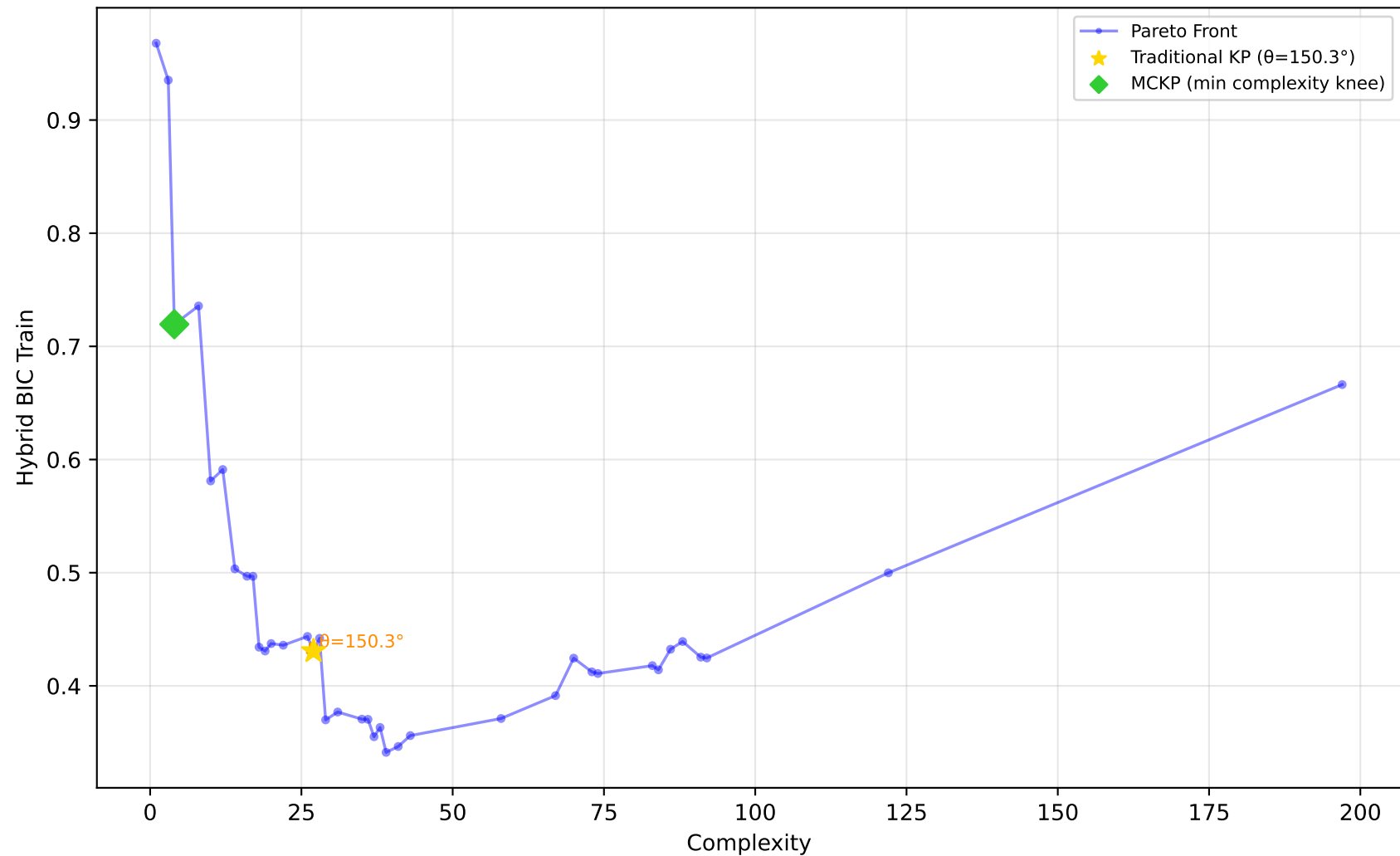
605_fri_c2_250_25 - Run 8 - MVP - Hybrid BIC Train \lambda_1=0.30, \lambda_2=0.00, \lambda_3=1.00 | Difficulty: 1.00 | Method: hmr
