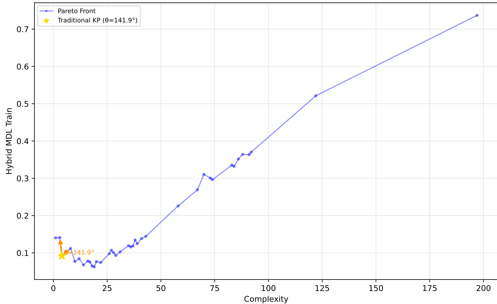
605_fri_c2_250_25 - Run 8 - MVP - Hybrid MDL Train \lambda_1=0.10, \lambda_2=0.00, \lambda_3=0.00 | Difficulty: 1.00 | Method: hmr
