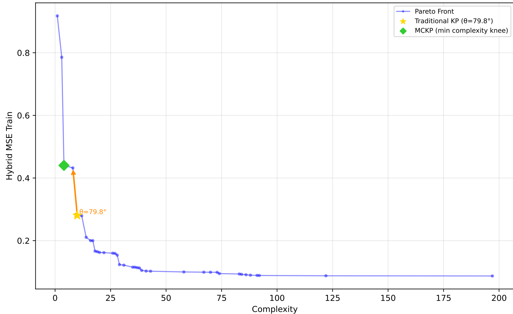
605_fri_c2_250_25 - Run 8 - MVP - Hybrid MSE Train \lambda_1=0.10, \lambda_2=0.00, \lambda_3=0.00 | Difficulty: 1.00 | Method: hmr
