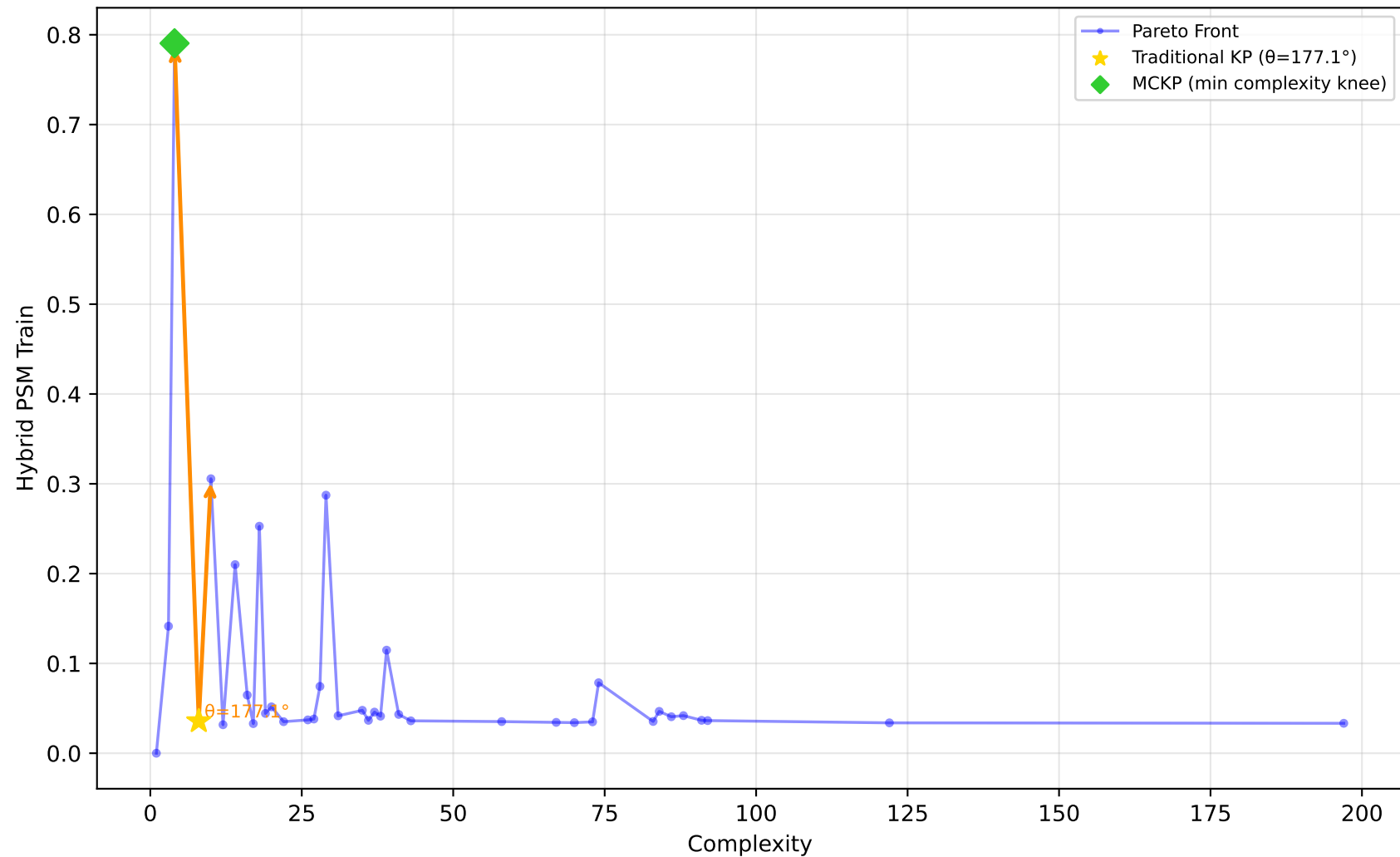
605_fri_c2_250_25 - Run 8 - MVP - Hybrid PSM Train \lambda_1=0.30, \lambda_2=0.00, \lambda_3=1.00 | Difficulty: 1.00 | Method: hmr
