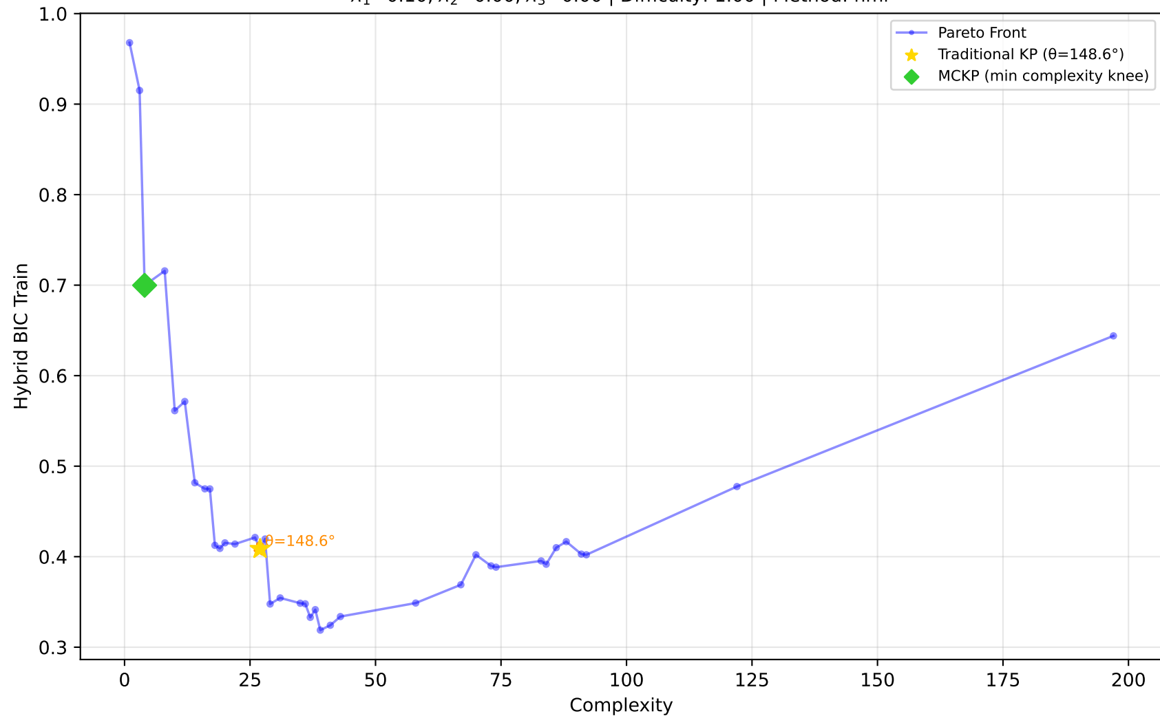
605_fri_c2_250_25 - Run 8 - SVP - Hybrid BIC Train \lambda_1=0.10, \lambda_2=0.00, \lambda_3=0.00 | Difficulty: 1.00 | Method: hmr
