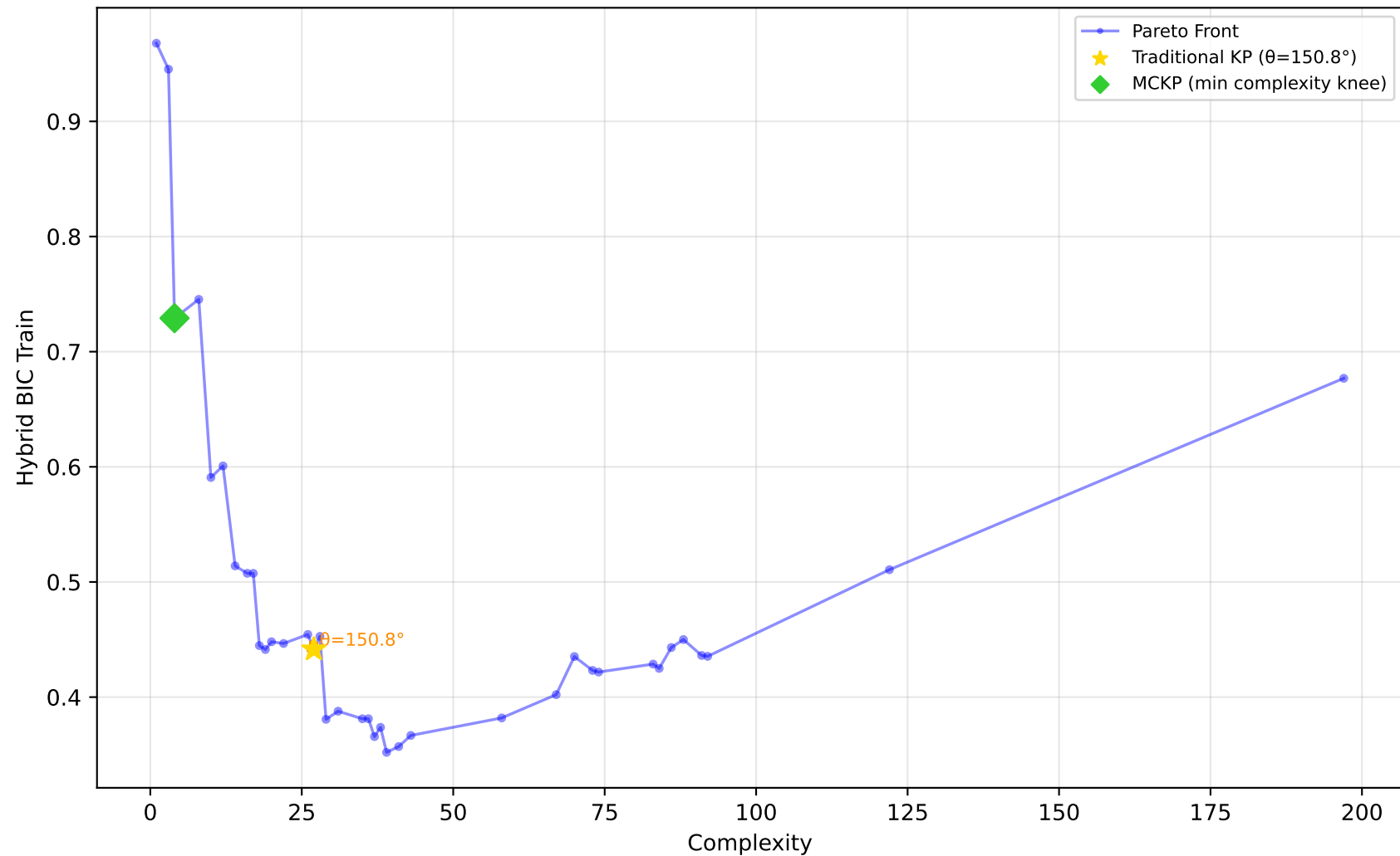
605_fri_c2_250_25 - Run 8 - SVP - Hybrid BIC Train \lambda_1=0.40, \lambda_2=0.00, \lambda_3=0.20 | Difficulty: 1.00 | Method: hmr
