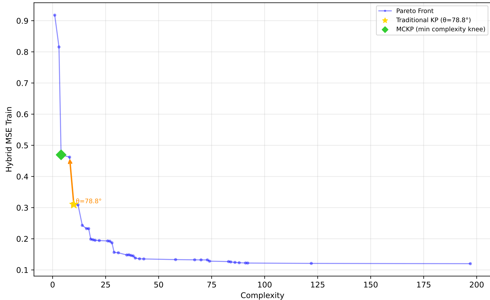
605_fri_c2_250_25 - Run 8 - SVP - Hybrid MSE Train \lambda_1=0.40, \lambda_2=0.00, \lambda_3=0.20 | Difficulty: 1.00 | Method: hmr
