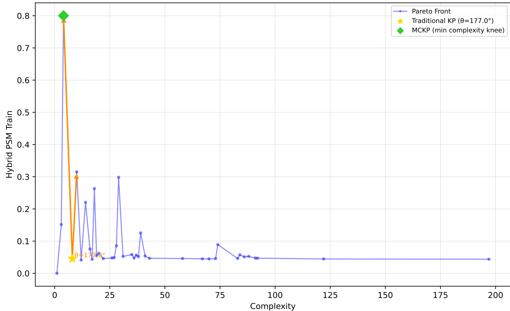
605_fri_c2_250_25 - Run 8 - SVP - Hybrid PSM Train \lambda_1=0.40, \lambda_2=0.00, \lambda_3=0.20 | Difficulty: 1.00 | Method: hmr
